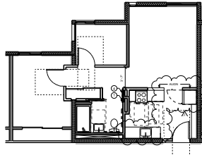
1 UNIT TYPE D - NEW CONSTRUCTION 10' x 10' WITH TUB TOTAL - 6 UNITS
