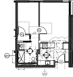
3 UNIT TYPE C MOBILITY - NEW CONSTRUCTION 10' x 10' WITH ACCESSIBLE ROLL-IN SHOWER TOTAL - 14 UNITS
