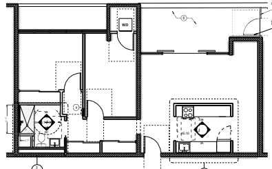
5 UNIT TYPE E (MOBILITY) - NEW CONSTRUCTION 10' x 10' WITH ACCESSIBLE ROLL-IN SHOWER TOTAL - 2 UNITS
