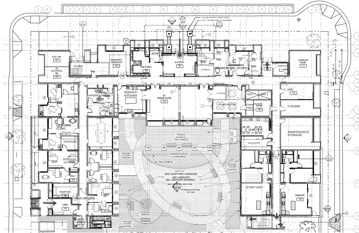
LEVEL T FLOOR PLAN PHASE I RENOVATIONS
