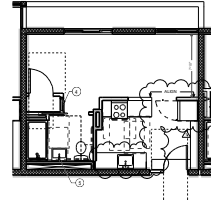
4 UNIT TYPE B - NEW CONSTRUCTION 10' x 10' WITH TUB TOTAL - 10 UNITS
