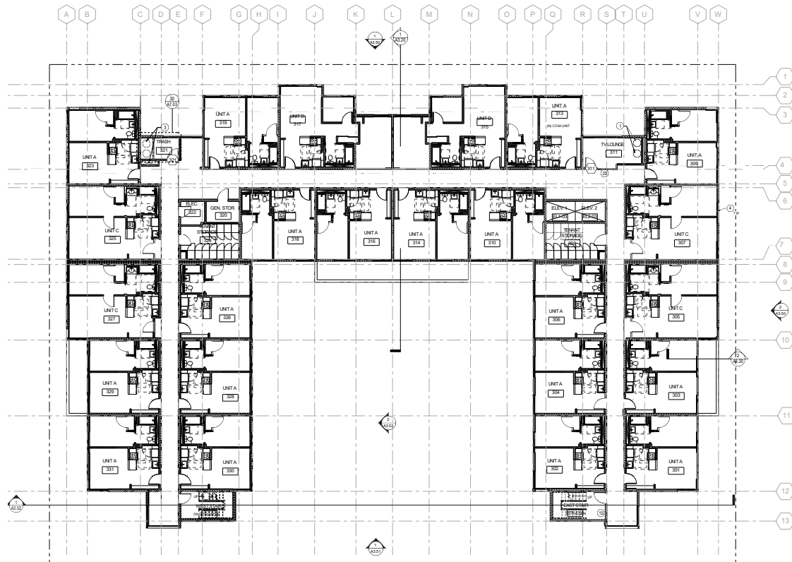
TYPICAL UPPER LEVEL FLOOR PLAN PHASE I RENOVATIONS
