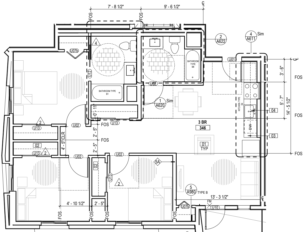
ENLARGED UNIT PLAN - 3BR - UNIT TYPE G 1/4" = 1'-0"
