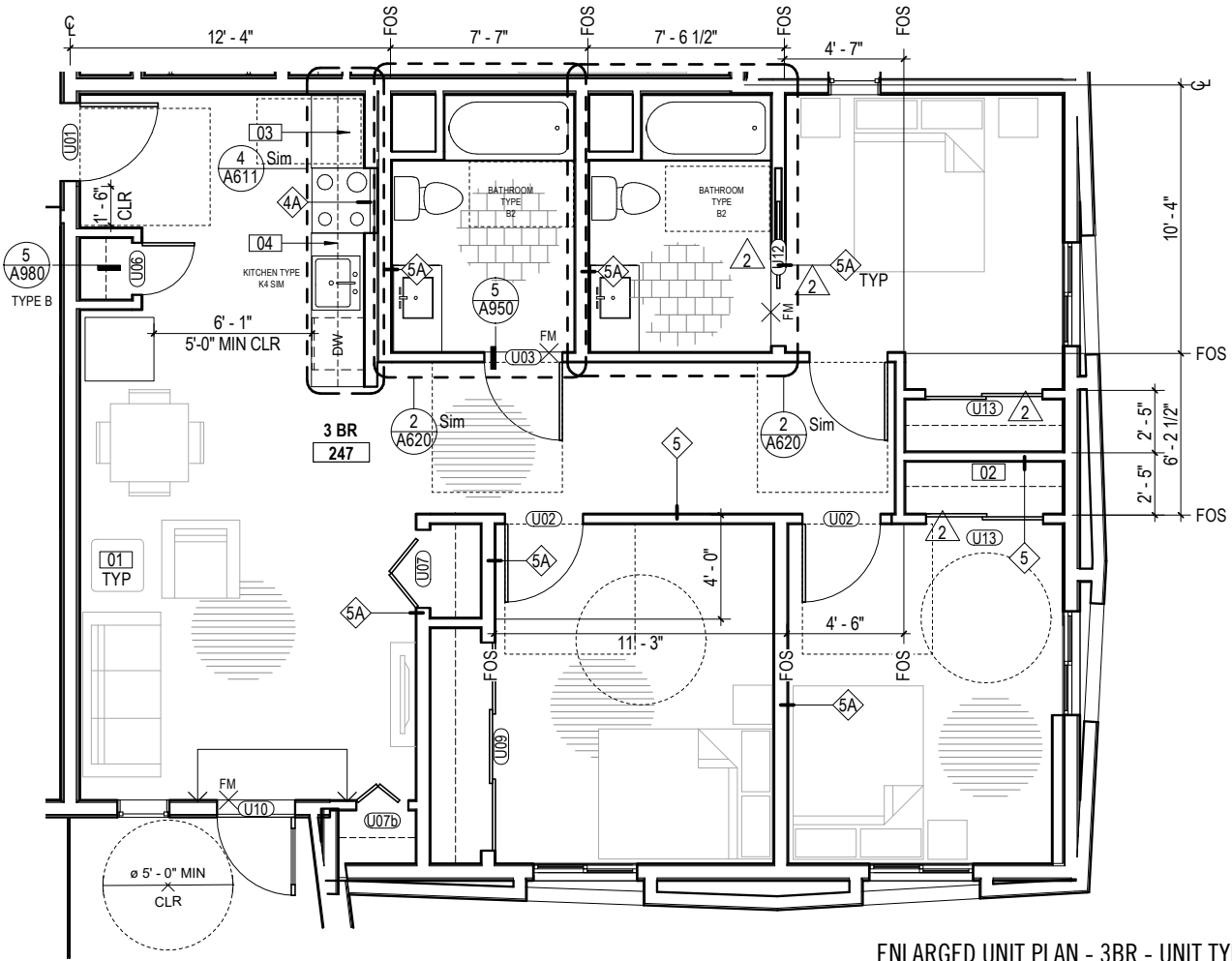
ENLARGED UNIT PLAN - 3BR - UNIT TYPE F 1/4" = 1'-0"
