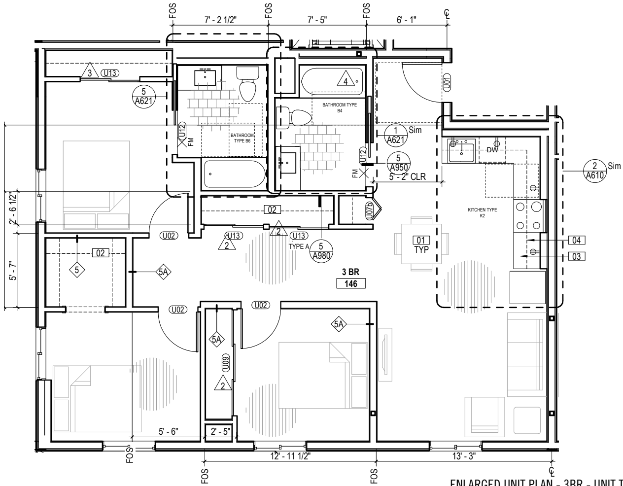
ENLARGED UNIT PLAN - 3BR - UNIT TYPE H 1/4" = 1'-0"
