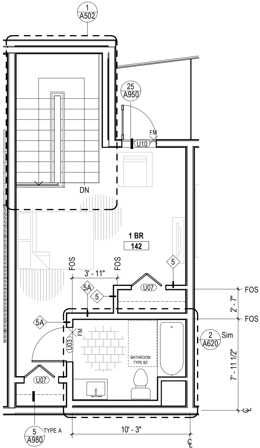
ENLARGED UNIT PLAN - 1BR - UNIT TYPE I 2F 1/4" = 1'-0"
