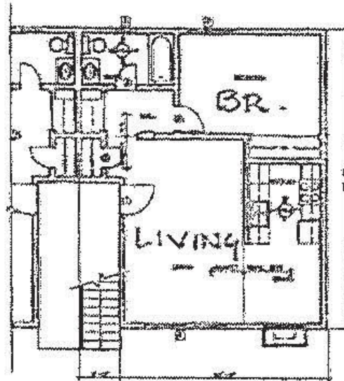
① FIRST FLOOR PLAN
