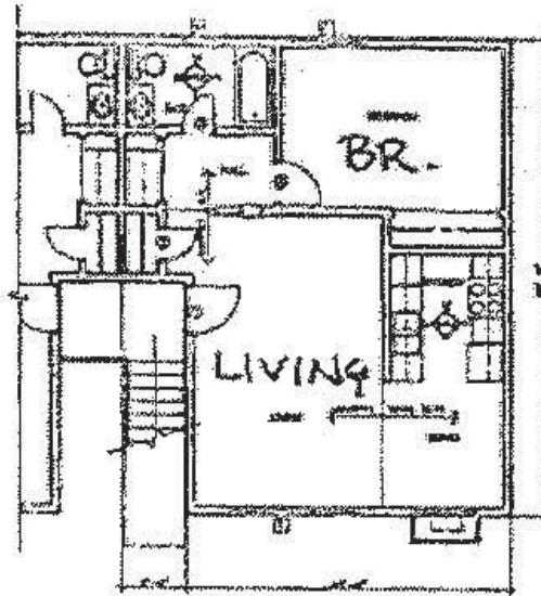
② SECOND FLOOR PLAN
